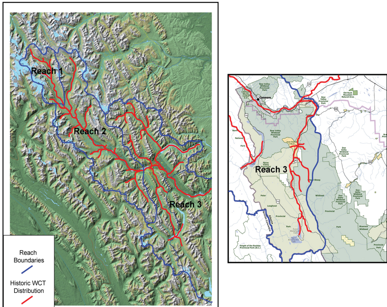
Figure 5. Historic distribution of westslope cutthroat trout in the Study Area. Base maps provided by Parks Canada and the Province of Alberta. Distribution data were modified from Mayhood, 1995.
