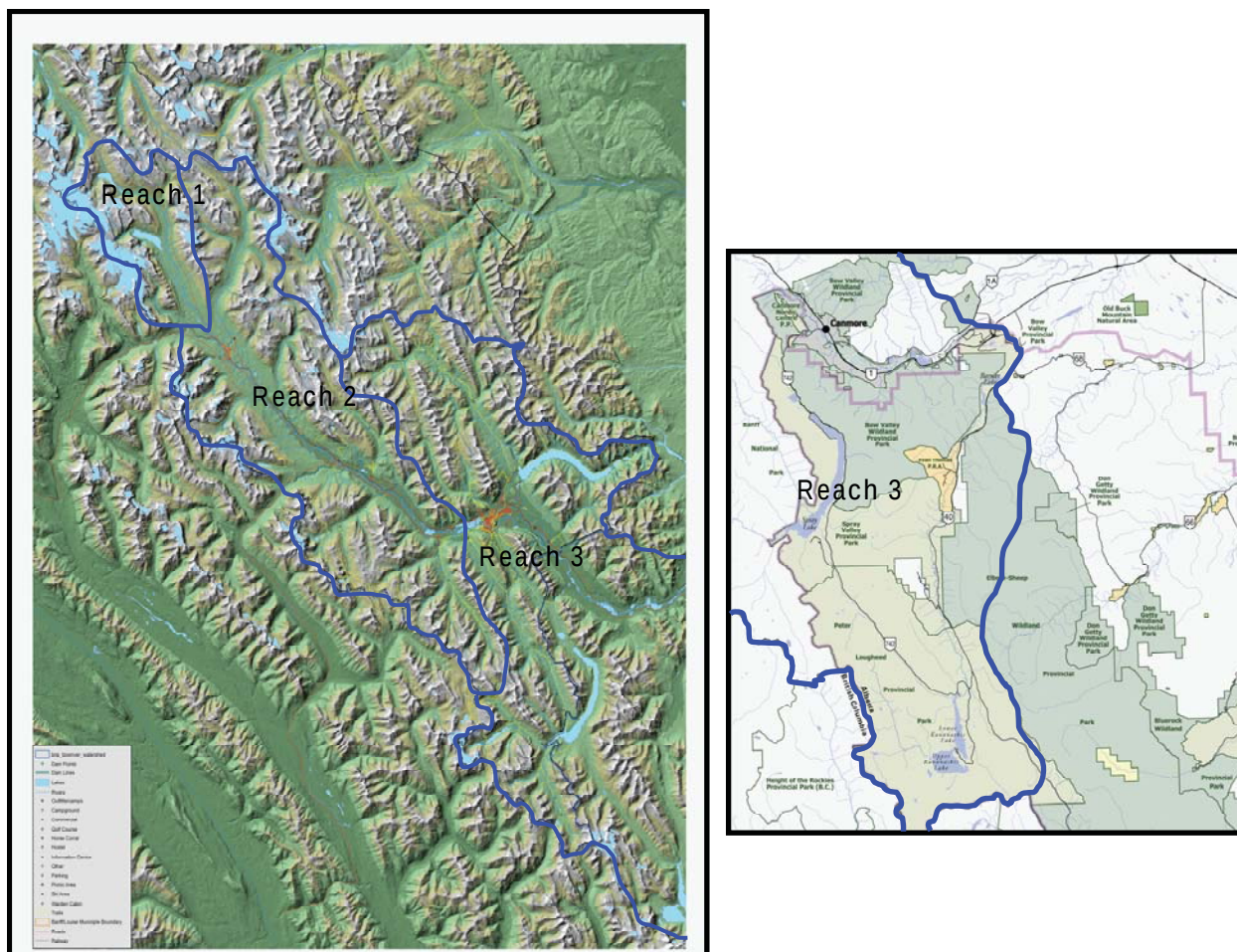
Figure 1. Boundaries for watersheds within each of the Reaches. Base maps provided by Parks Canada and the Province of Alberta.
