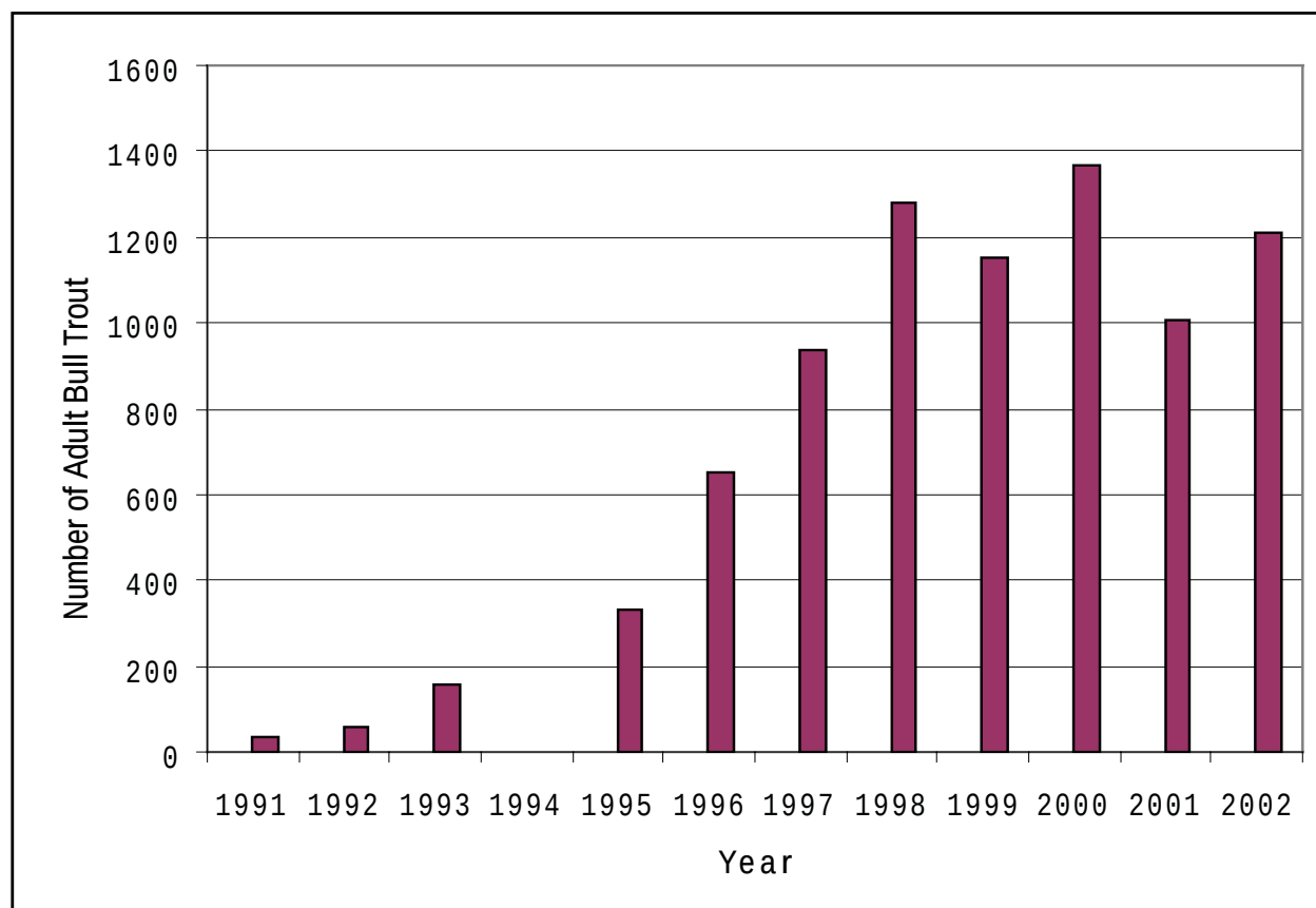
Figure 4. Number of bull trout captured in a weir trap in Smith-Dorrien Creek. Data from the Province of Alberta.
